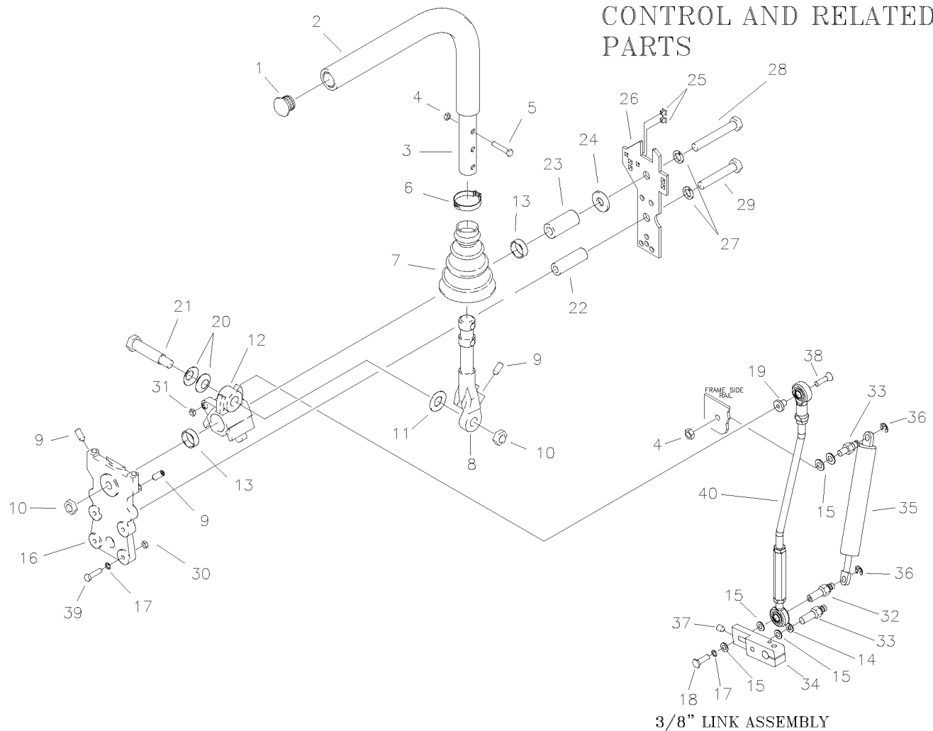
3/8" LINK ASSEMBLY
