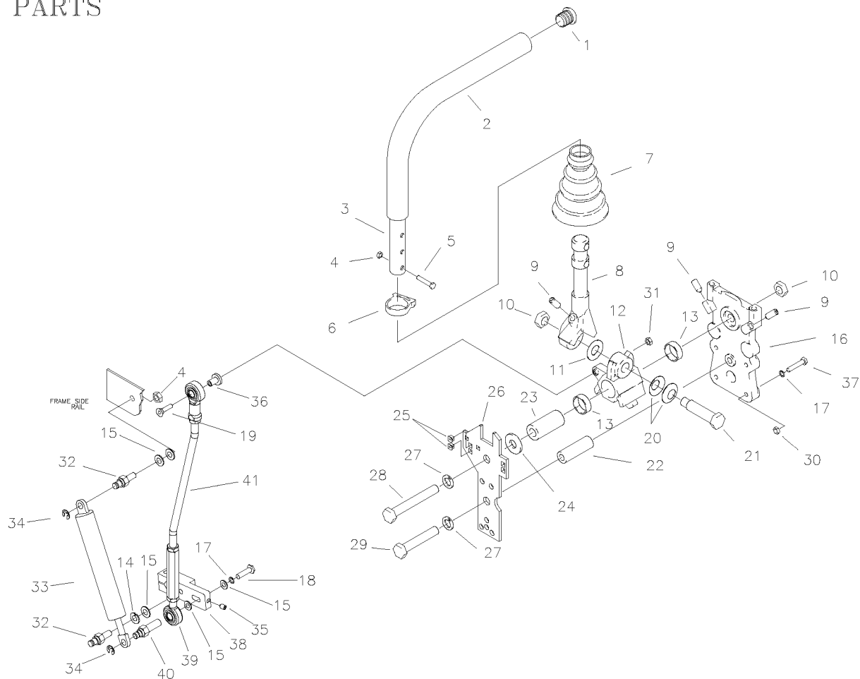
3/8" LINK ASSEMBLY
