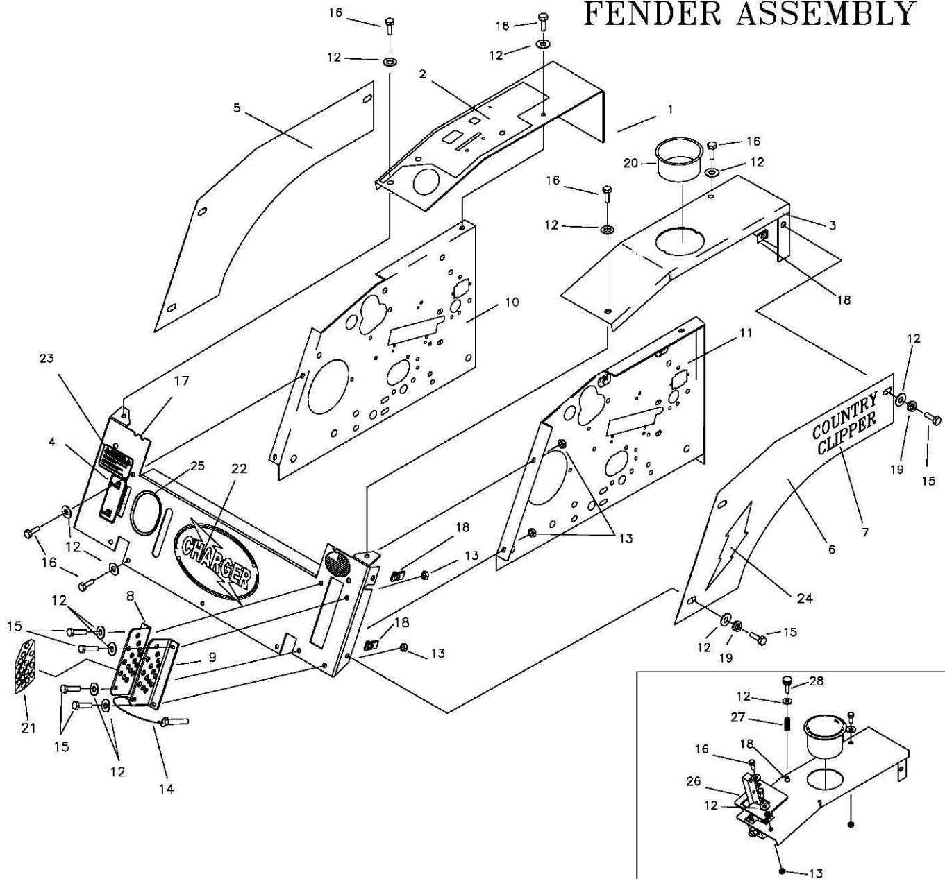
TWINSTICK FENDER ASSY
