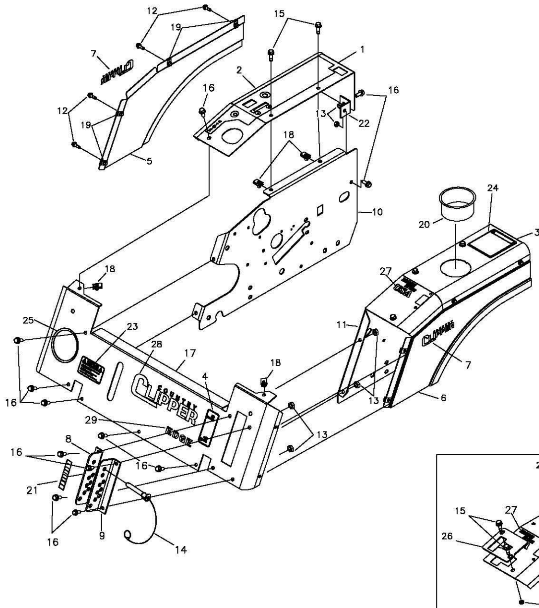
TWINSTICK FENDER ASSY
